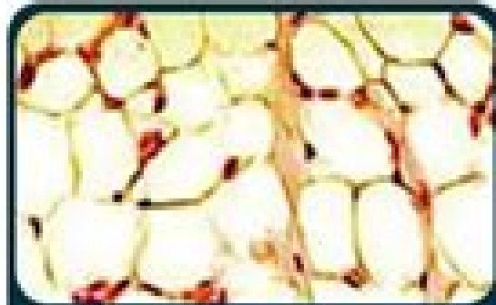
Adipose tissue
