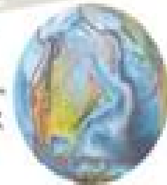
1 The plates are moving in different directions. 2 The plates are moving in the same direction. 3 The plates are moving in opposite directions. 4 The plates are moving in the same direction. 5 The plates are moving in opposite directions. 6 The plates are moving in the same direction. 7 The plates are moving in opposite directions. 8 The plates are moving in the same direction. 9 The plates are moving in opposite directions. 10 The plates are moving in the same direction. 11 The plates are moving in opposite directions. 12 The plates are moving in the same direction. 13 The plates are moving in opposite directions. 14 The plates are moving in the same direction. 15 The plates are moving in opposite directions. 16 The plates are moving in the same direction. 17 The plates are moving in opposite directions. 18 The plates are moving in the same direction. 19 The plates are moving in opposite directions. 20 The plates are moving in the same direction. 21 The plates are moving in opposite directions. 22 The plates are moving in the same direction. 23 The plates are moving in opposite directions. 24 The plates are moving in the same direction. 25 The plates are moving in opposite directions. 26 The plates are moving in the same direction. 27 The plates are moving in opposite directions. 28 The plates are moving in the same direction. 29 The plates are moving in opposite directions. 30 The plates are moving in the same direction. 31 The plates are moving in opposite directions. 32 The plates are moving in the same direction. 33 The plates are moving in opposite directions. 34 The plates are moving in the same direction. 35 The plates are moving in opposite directions. 36 The plates are moving in the same direction. 37 The plates are moving in opposite directions. 38 The plates are moving in the same direction. 39 The plates are moving in opposite directions. 40 The plates are moving in the same direction. 41 The plates are moving in opposite directions. 42 The plates are moving in the same direction. 43 The plates are moving in opposite directions. 44 The plates are moving in the same direction. 45 The plates are moving in opposite directions. 46 The plates are moving in the same direction. 47 The plates are moving in opposite directions. 48 The plates are moving in the same direction. 49 The plates are moving in opposite directions. 50 The plates are moving in the same direction. 51 The plates are moving in opposite directions. 52 The plates are moving in the same direction. 53 The plates are moving in opposite directions. 54 The plates are moving in the same direction. 55 The plates are moving in opposite directions. 56 The plates are moving in the same direction. 57 The plates are moving in opposite directions. 58 The plates are moving in the same direction. 59 The plates are moving in opposite directions. 60 The plates are moving in the same direction. 61 The plates are moving in opposite directions. 62 The plates are moving in the same direction. 63 The plates are moving in opposite directions. 64 The plates are moving in the same direction. 65 The plates are moving in opposite directions. 66 The plates are moving in the same direction. 67 The plates are moving in opposite directions. 68 The plates are moving in the same direction. 69 The plates are moving in opposite directions. 70 The plates are moving in the same direction. 71 The plates are moving in opposite directions. 72 The plates are moving in the same direction. 73 The plates are moving in opposite directions. 74 The plates are moving in the same direction. 75 The plates are moving in opposite directions. 76 The plates are moving in the same direction. 77 The plates are moving in opposite directions. 78 The plates are moving in the same direction. 79 The plates are moving in opposite directions. 80 The plates are moving in the same direction. 81 The plates are moving in opposite directions. 82 The plates are moving in the same direction. 83 The plates are moving in opposite directions. 84 The plates are moving in the same direction. 85 The plates are moving in opposite directions. 86 The plates are moving in the same direction. 87 The plates are moving in opposite directions. 88 The plates are moving in the same direction. 89 The plates are moving in opposite directions. 90 The plates are moving in the same direction. 91 The plates are moving in opposite directions. 92 The plates are moving in the same direction. 93 The plates are moving in opposite directions. 94 The plates are moving in the same direction. 95 The plates are moving in opposite directions. 96 The plates are moving in the same direction. 97 The plates are moving in opposite directions. 98 The plates are moving in the same direction. 99 The plates are moving in opposite directions. 100 The plates are moving in the same direction.
