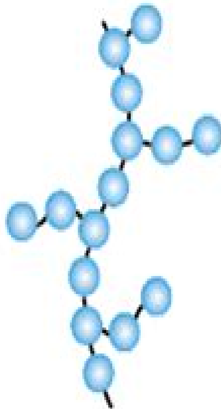
Branched
