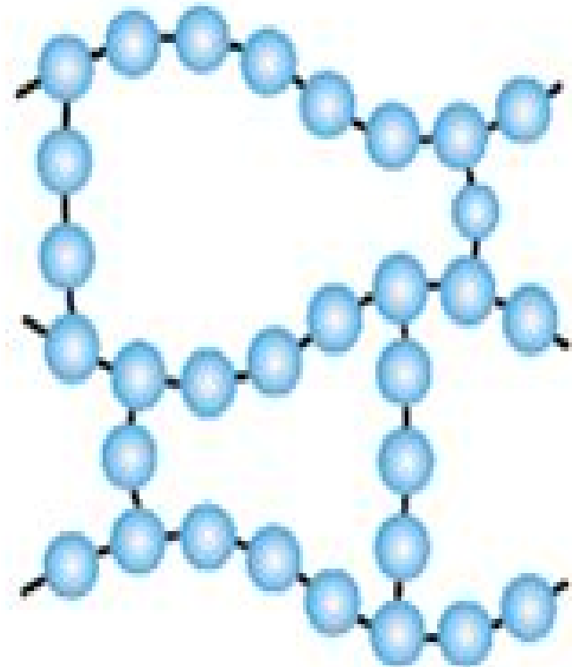
Cross-linked
