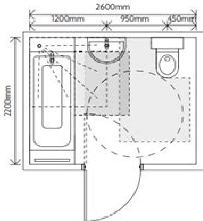
Example 3.15A – wheelchair adaptable bathroom (based on wheelchair accessible layout 3.16A)
