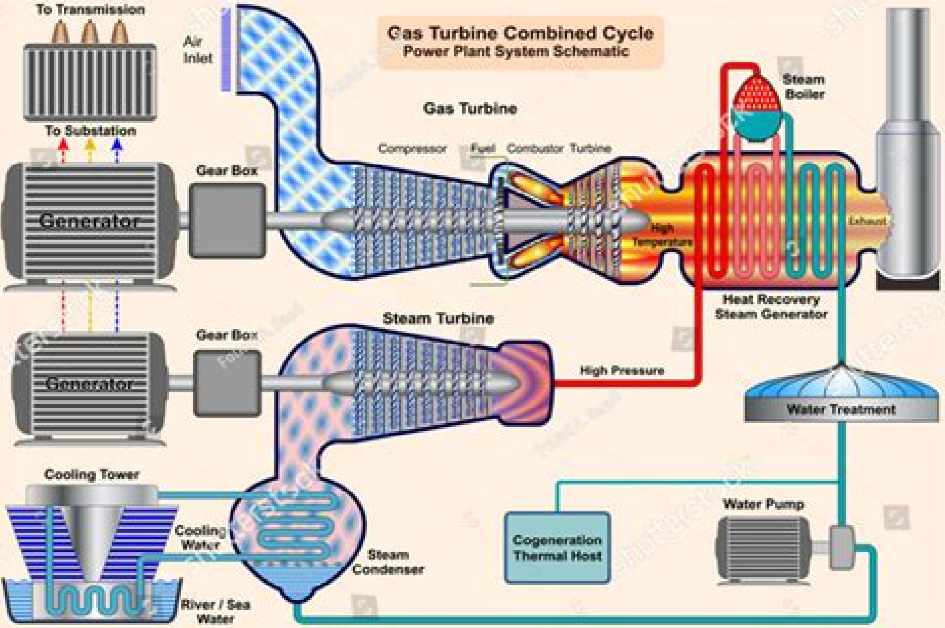
Vector Gas Turbine Combined Cycle EPS 10
