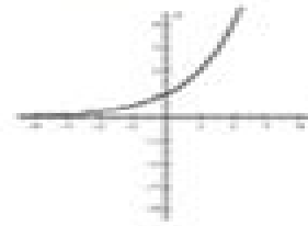
Exponential
