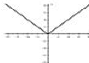
Absolute Value
