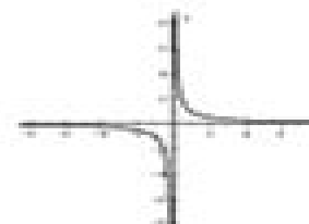
Reciprocal/Inverse/ Rational
