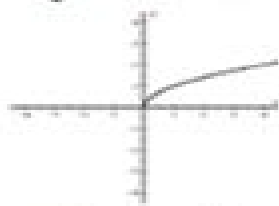
Square Root
