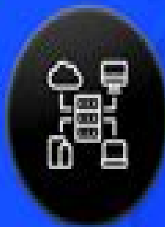
Network Database
