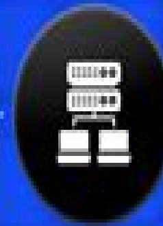
Object-Oriented Database
