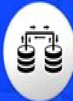
Relational Database
