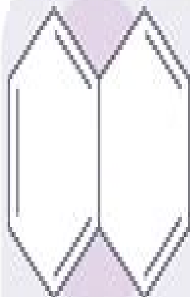
Naphthalene
