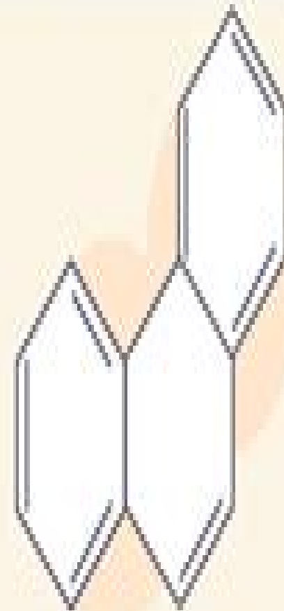
Phenanthrene
