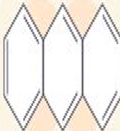
Anthracene
