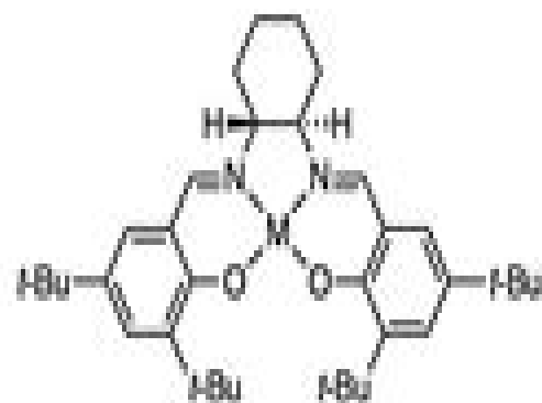
salen complexes
