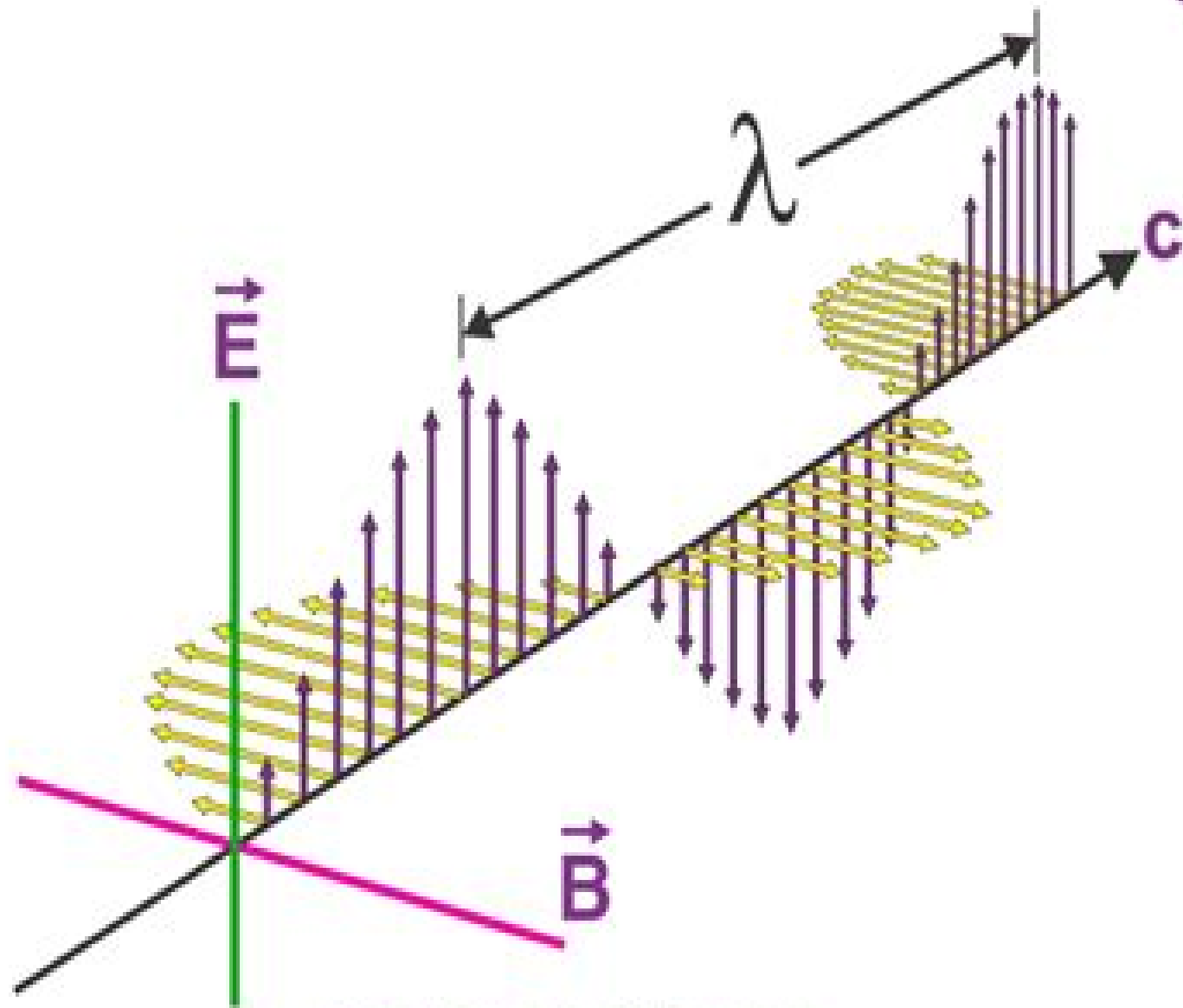
Electromagnetic wave
