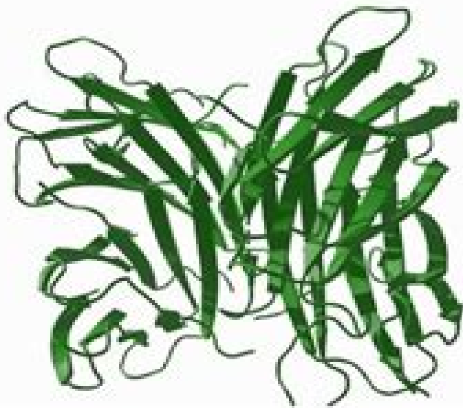
beta sheet
