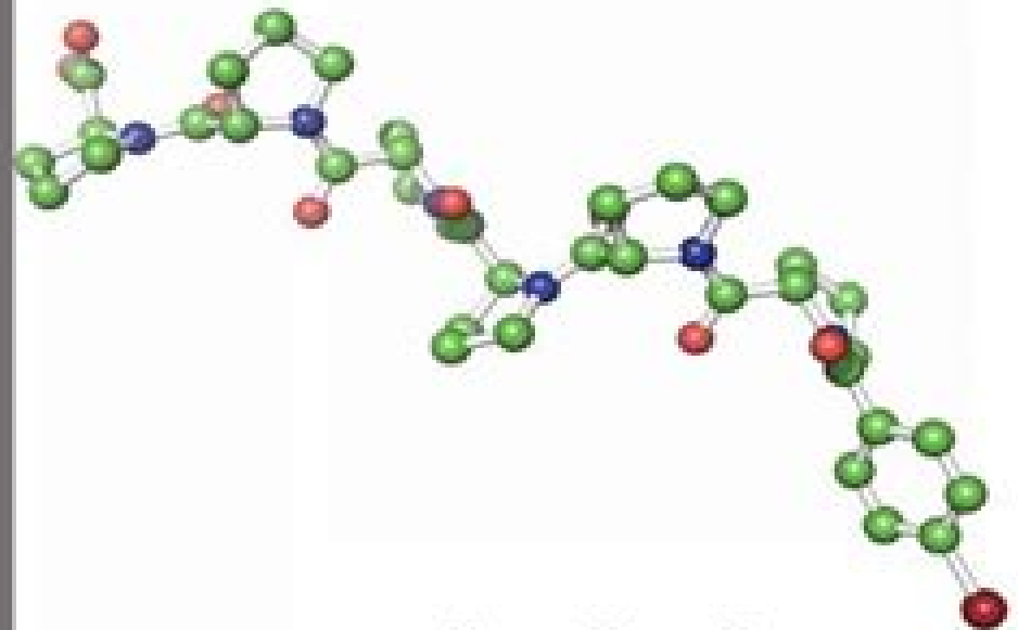
polyproline II
