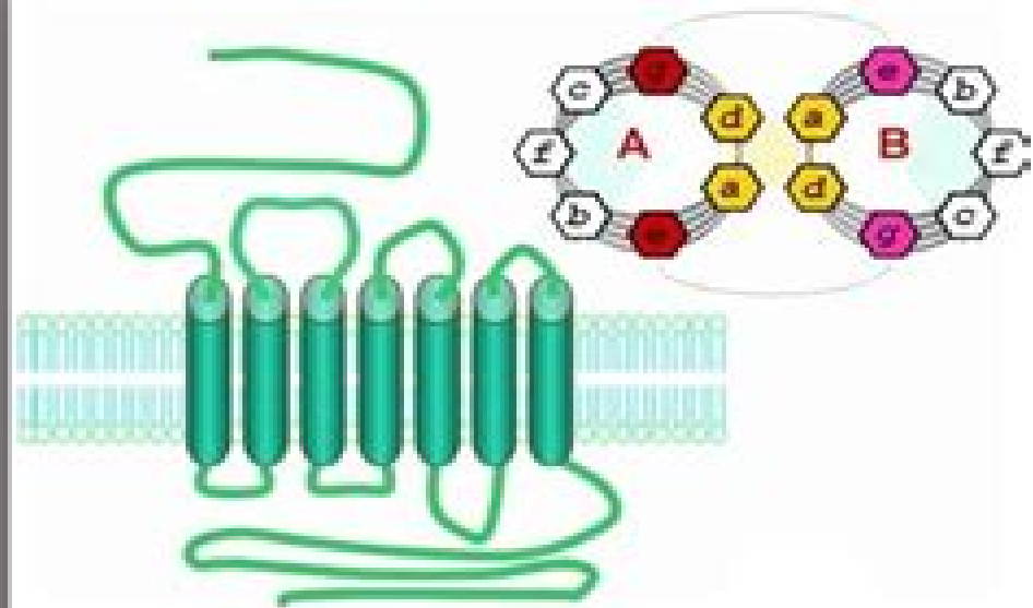
amphipathic helix
