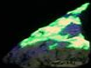
Hyalite Opal
