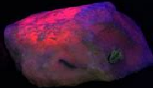
Fluorite
