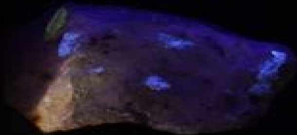
Gold Ore
