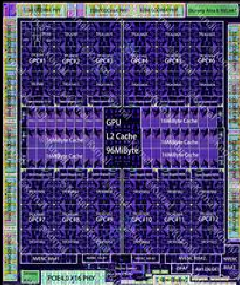
AD102 23.37mm x 26.36mm
