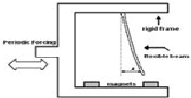
Figure 1. Mechanical interpretation of Duffing oscillator.
