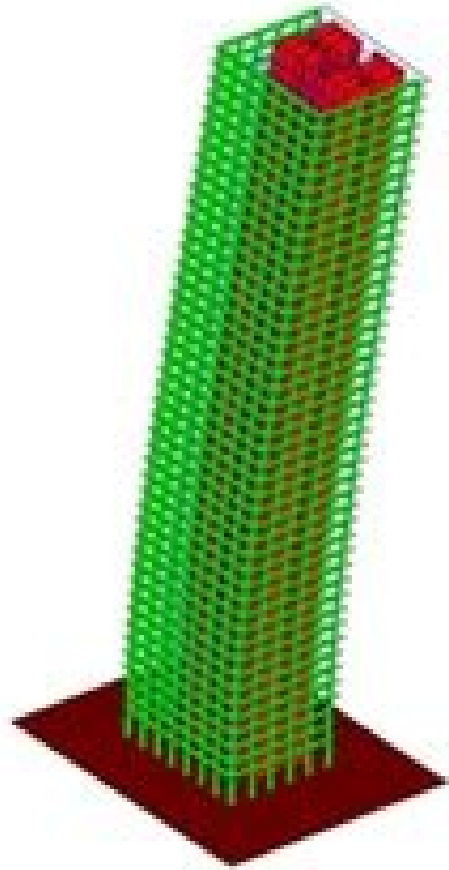
1 st Mode Shape: 0.18 Hz
