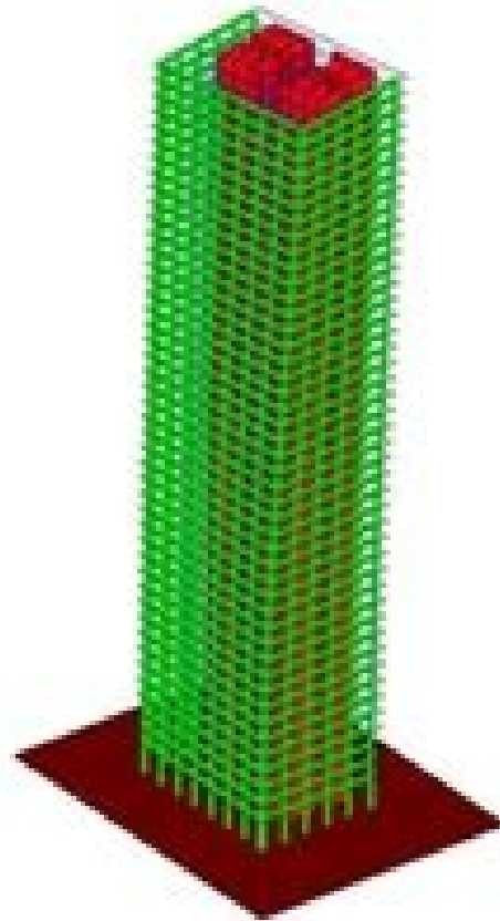
2 nd Mode Shape: 0.20 Hz
