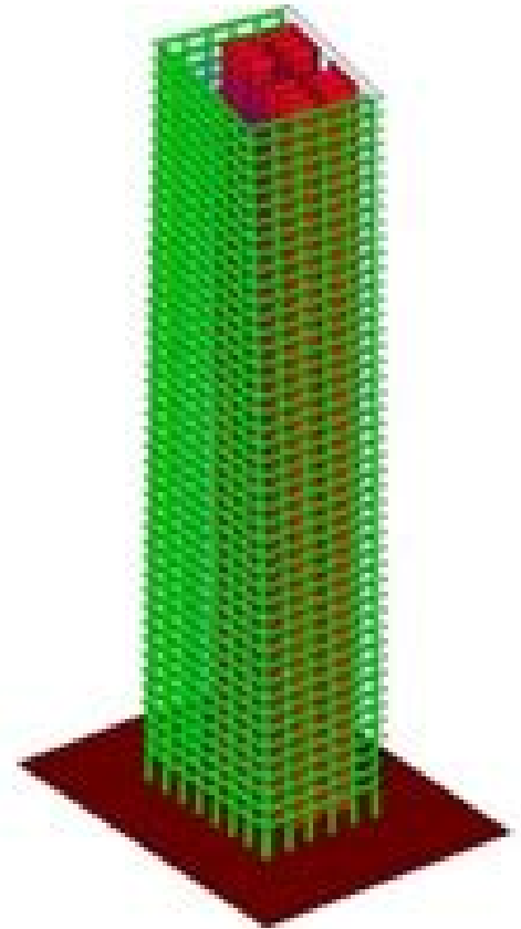
3 rd Mode Shape: 0.58 Hz
