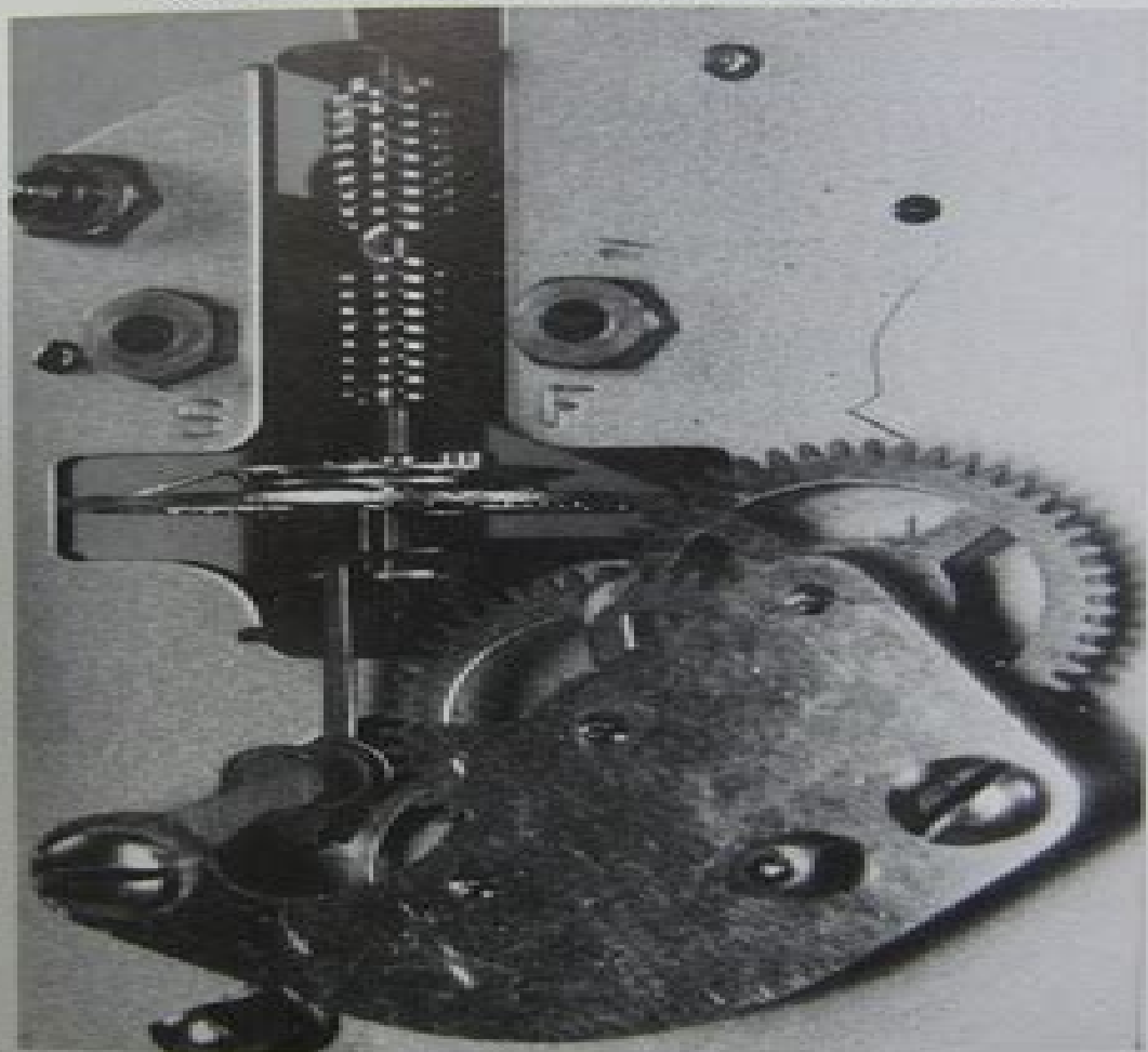
Plate 1 Floating balance and pin-pallet escapement
