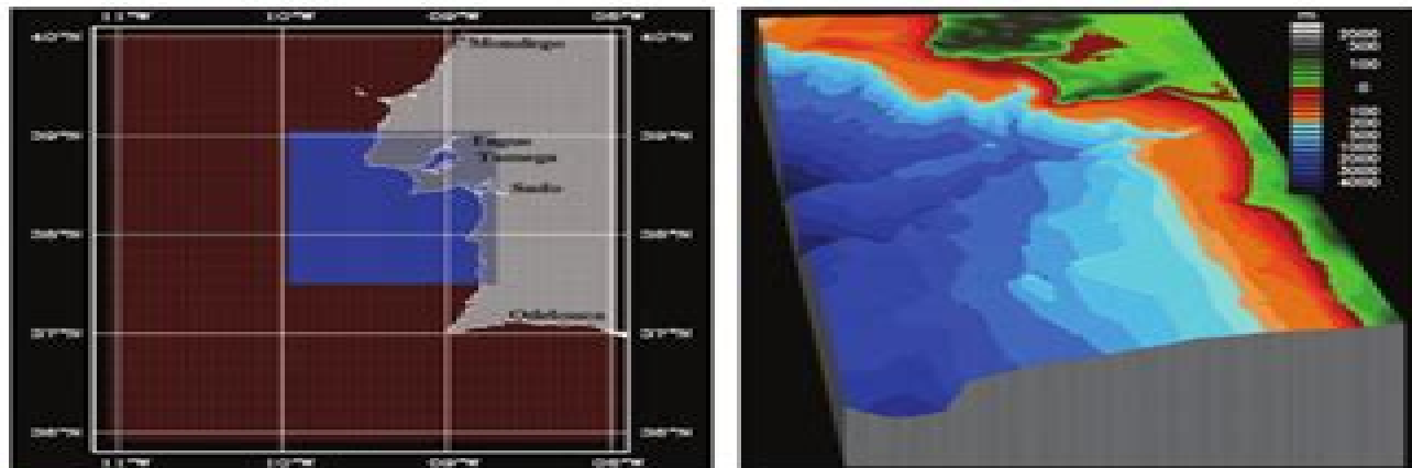
FIGURE 1 Left: Nested NCOM grid for MREA04 Trial. Outer grid (red) has horizontal 4-km resolution inner grid (blue) has 1-km resolution. River discharge locations are annotated. Right: 3D depiction of model bathymetry (m) for 1-km NCOM nest. Note canyon feature that extends close to the coast.
