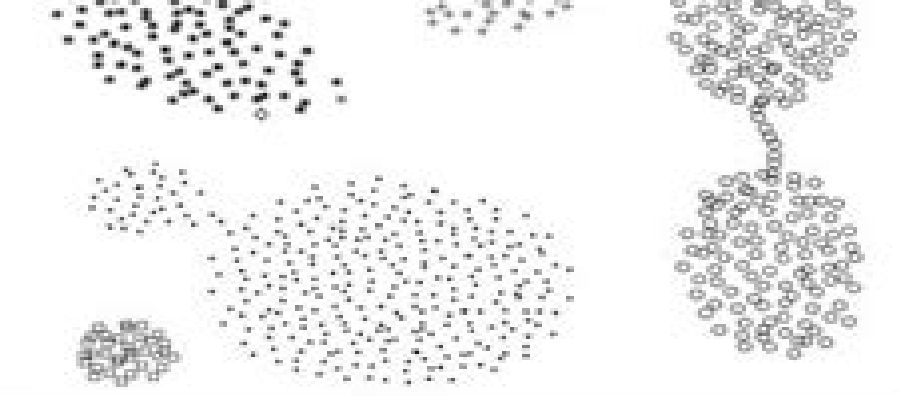
Average linkage
