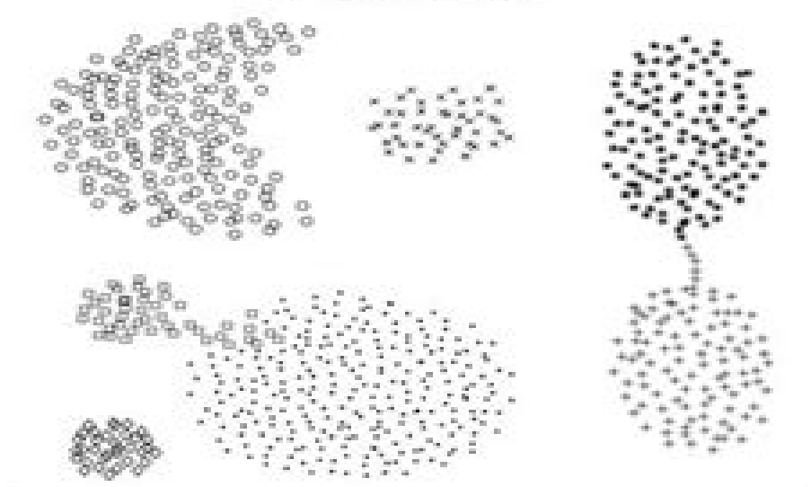
K-means
