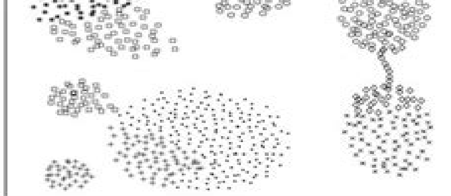
Ward's clustering
