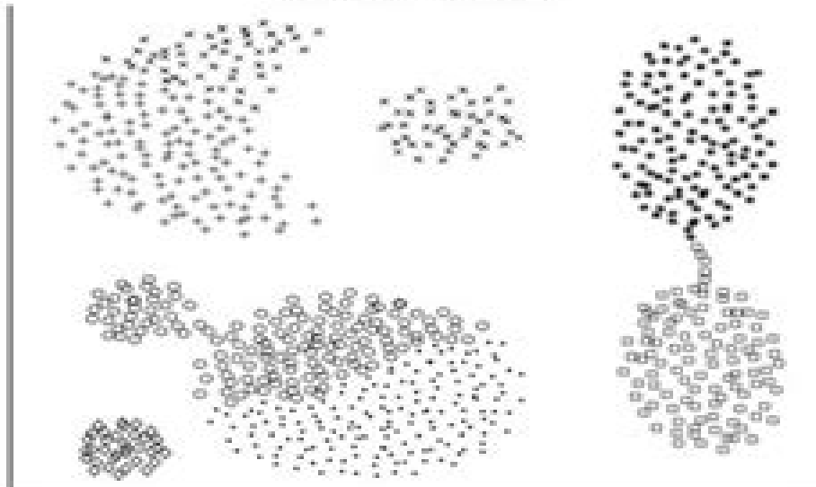
Clustering aggregation
