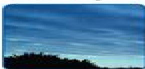
Stratus (spread out or layered)
