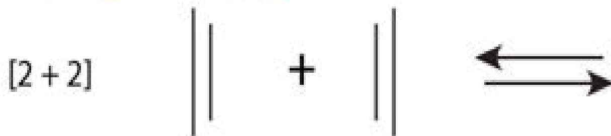
Ethylene
