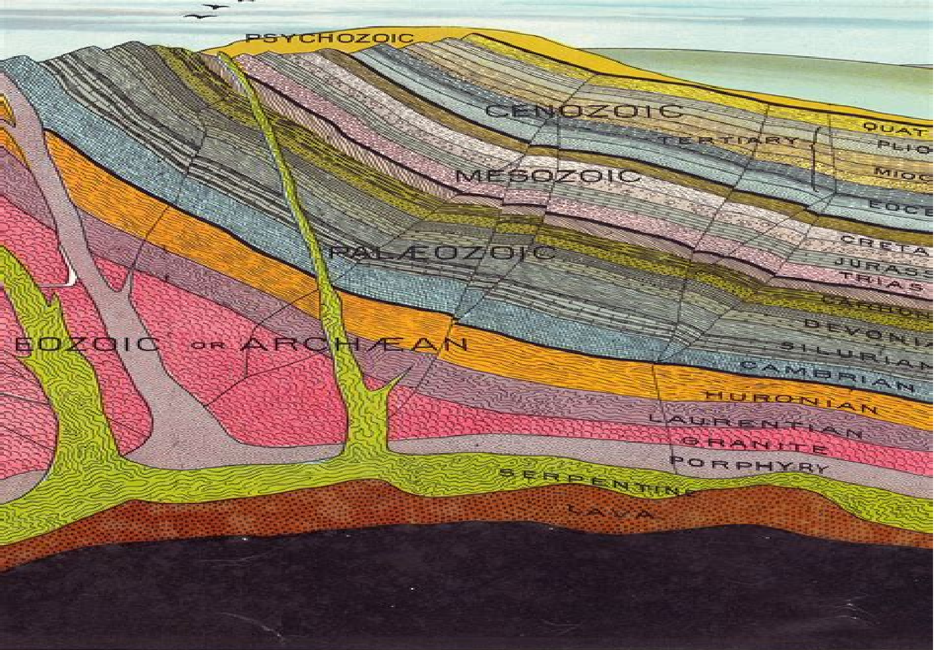
GEOLOGICAL CHART.
