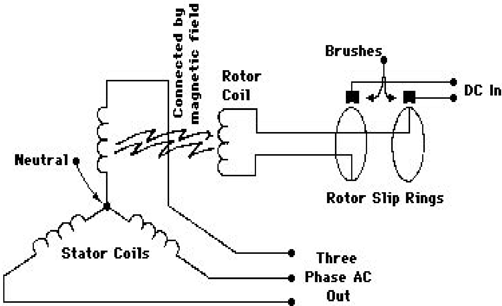
ELECTRICAL SCHEMATIC OF A TYPICAL ALTERNATOR
