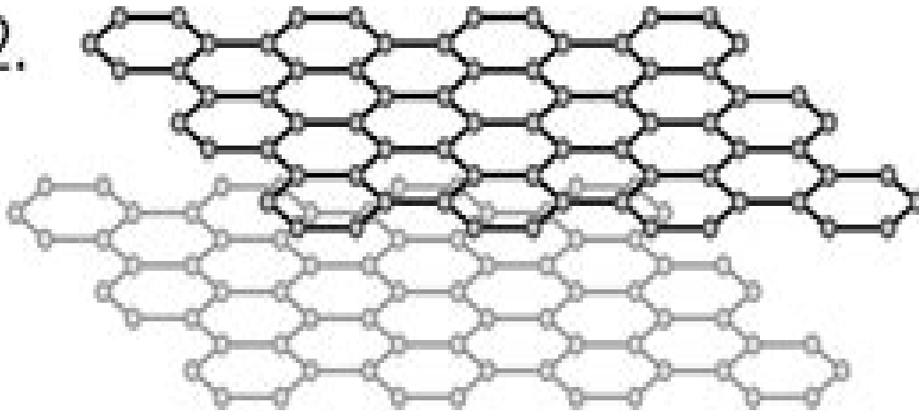
graphite
