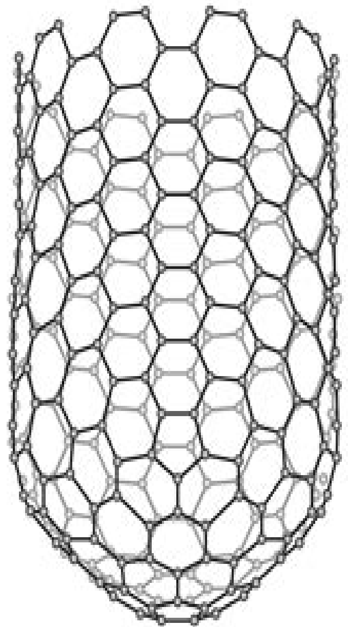
nanotube
