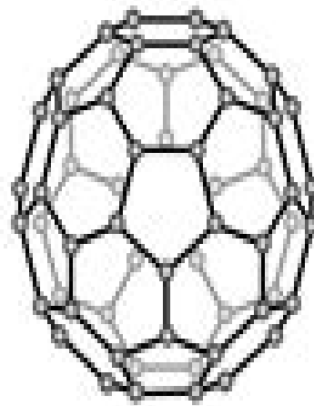
C 60 fullerene
