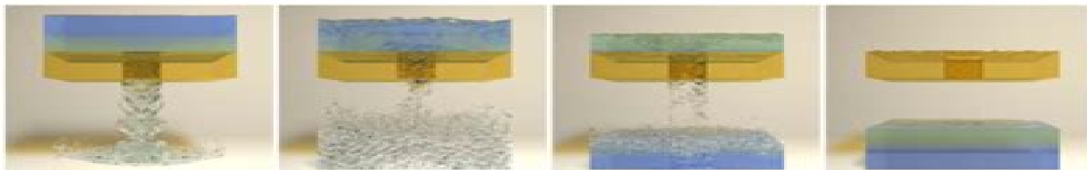
Fig. 1. Gugging with Rayleigh–Taylor instability: Our multiphase solver produces gugging for two-colored immiscible fluids in the transparent upper container and air in the bottom one (water-air with density ratios 100:100:1), with a square conduit in between. The two fluids are initially arranged with the heavier fluid (blue) on top of the lighter fluid (cyan), thus forming Rayleigh–Taylor instabilities early on, before flowing down and exhibiting splashes, bubbles and wetting, and ending up in stable layers based on their densities.
