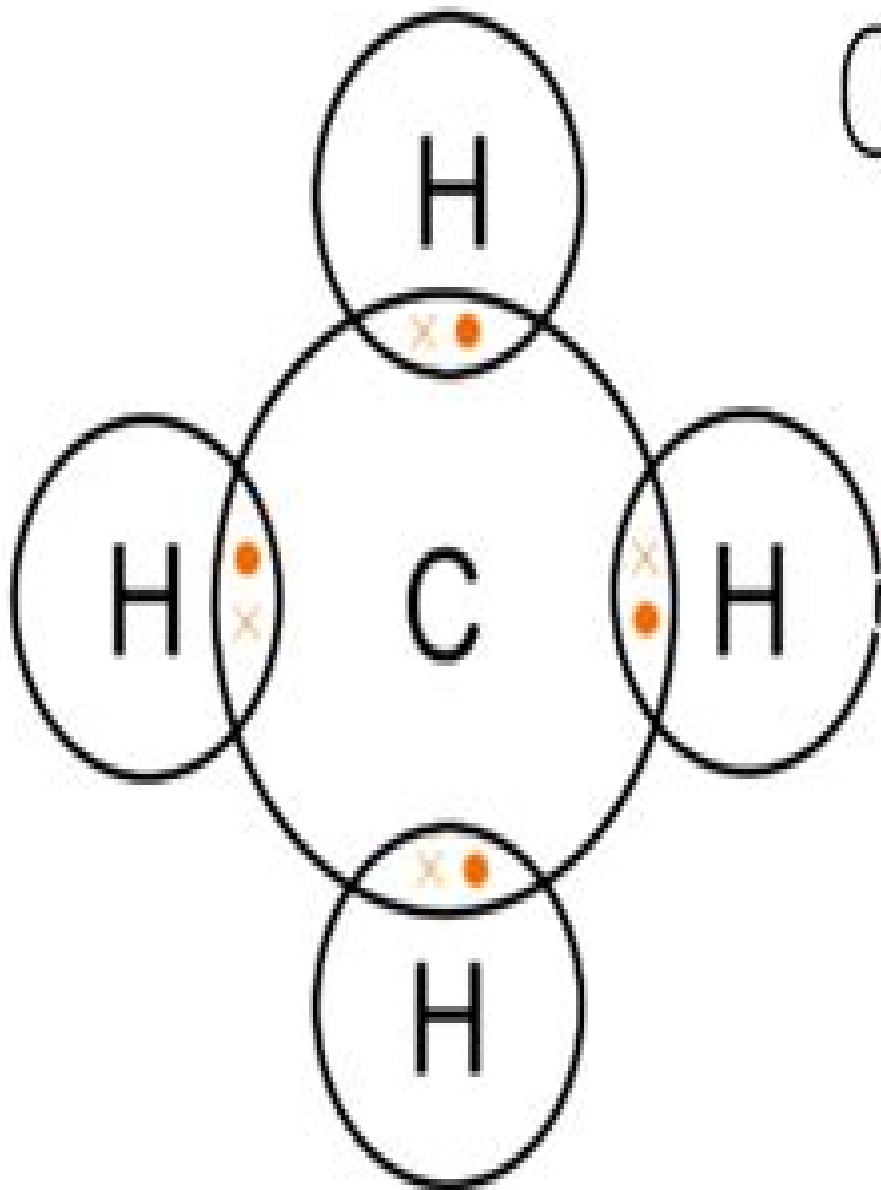
Carbon Hydrogen Bond
