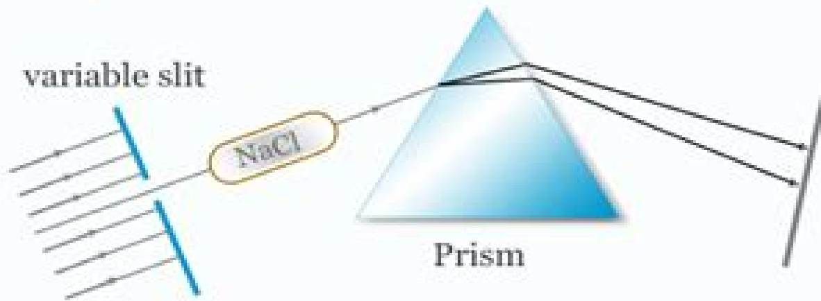
ABSORPTION SPECTRUM
