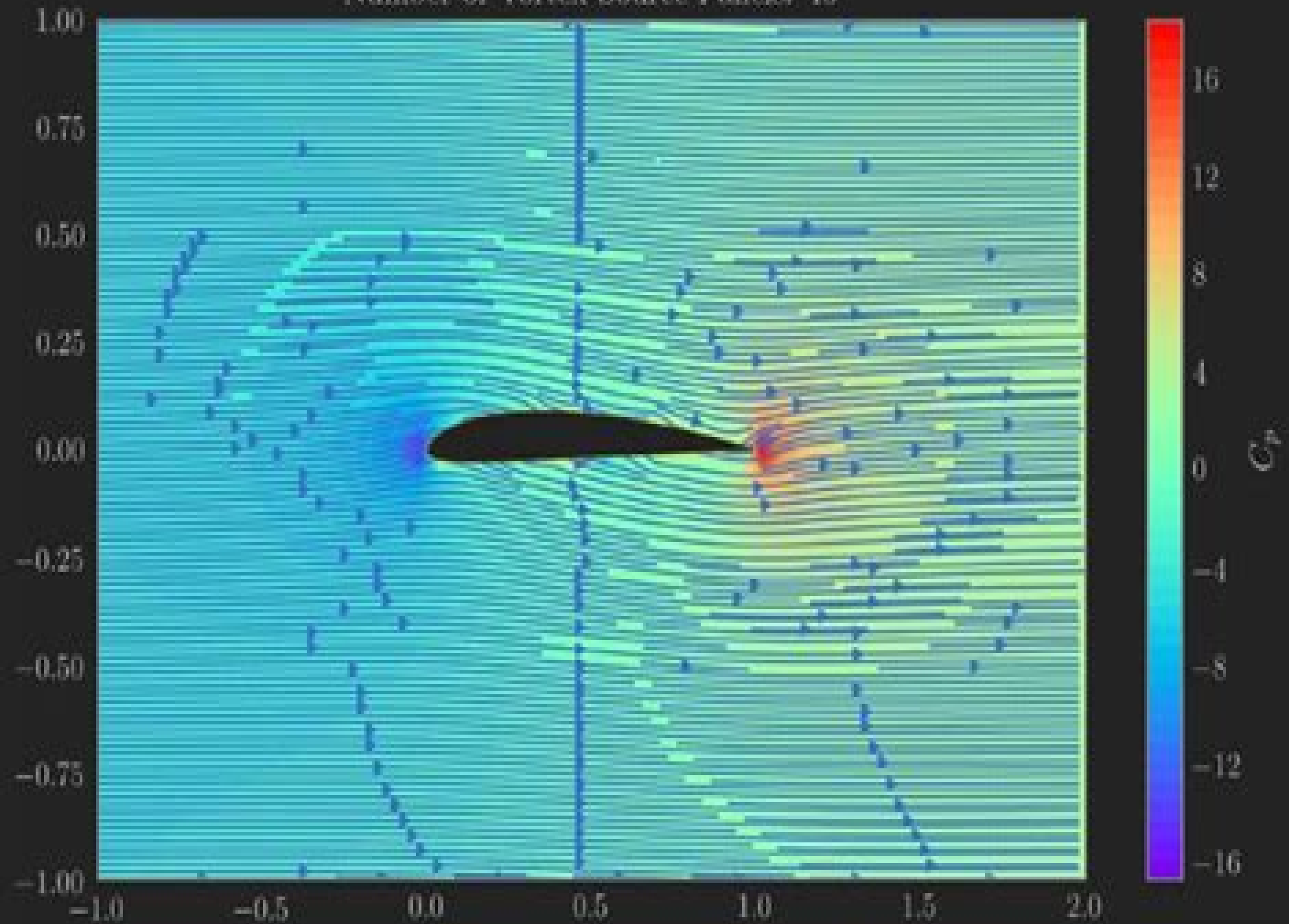
Number of Vortex-Source Panels: 40
