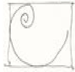
Fibonacci Spiral
