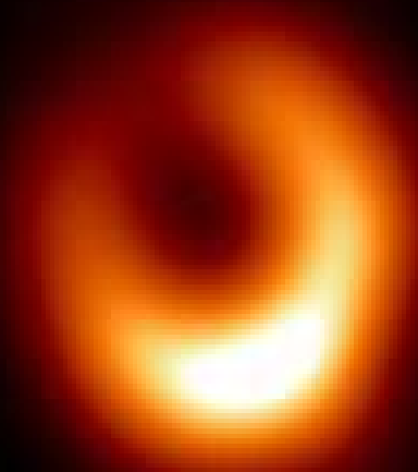
M87* April 21, 2018
