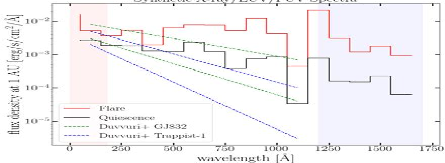
Synthetic X-ray/EUV/FUV Spectra
