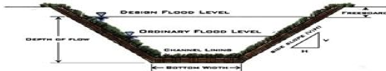
Figure 1: Typical Channel Cross Section
