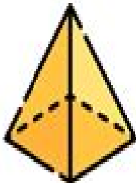
square pyramid
