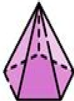
pentagonal pyramid
