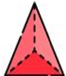
tetrahedron
