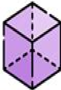
cube
