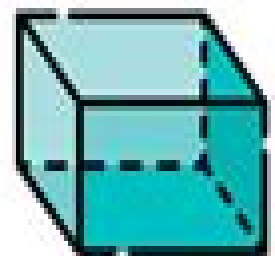
rectangular prism
