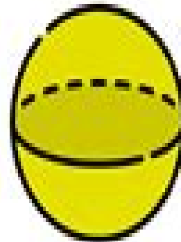
sphere
