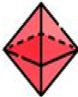
octahedron
