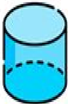
cylinder
