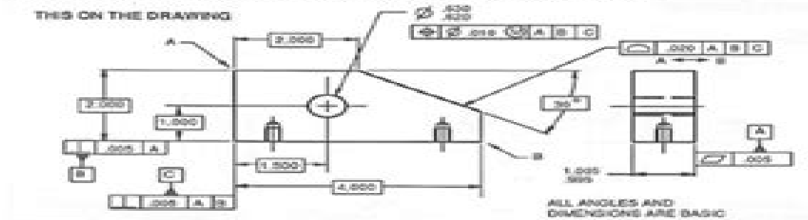
Figure 6-4. Fully toleranced design
