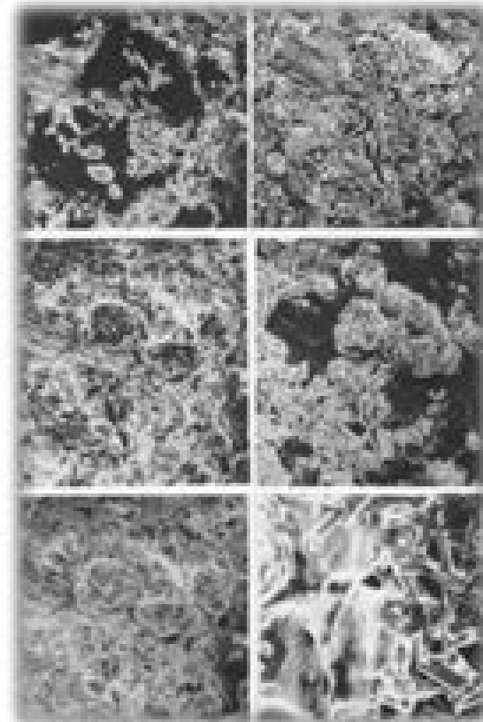
Corroded Surface of Sintered \text{YBa}_2\text{Cu}_3\text{O}_7 .
