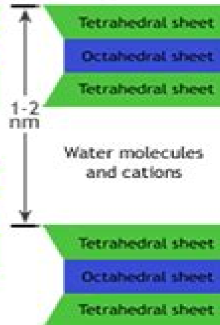
Smectite (2:1) Highly Expansive
