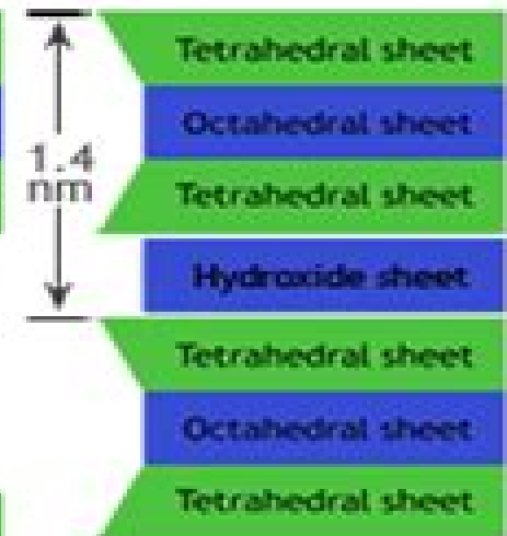
Chlorite (2:1) Nonexpansive
