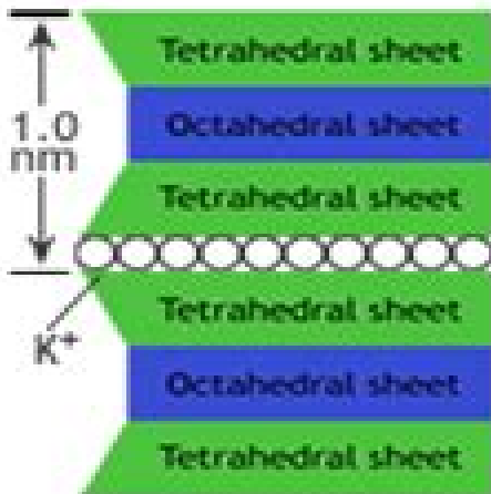
Illite (2:1) Nonexpansive
