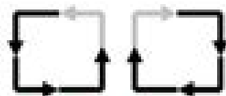
North-Last
