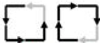
West-First
