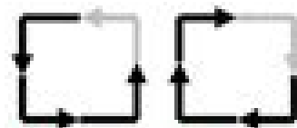
Negative-First
