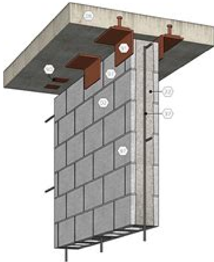
Masonry restraint at concrete slab
