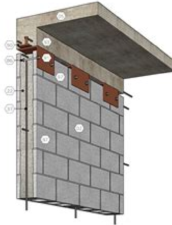
Masonry restraint at concrete beam
