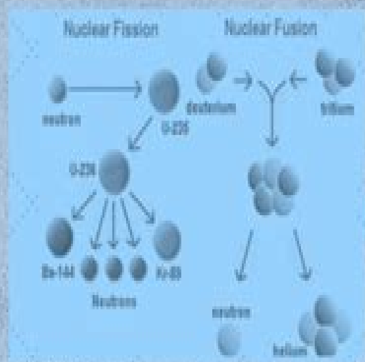
Nuclear reactions
