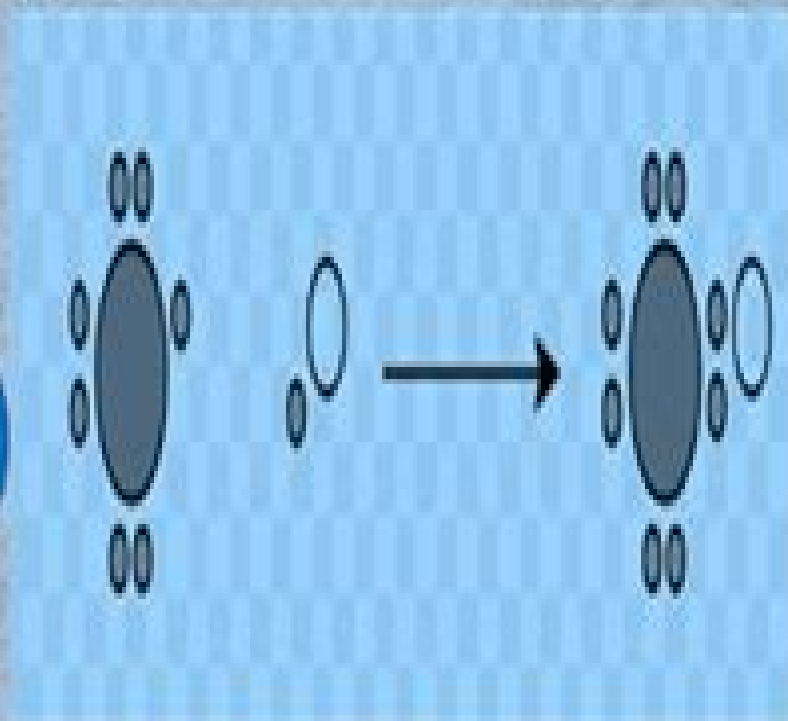
Chemical reactions
