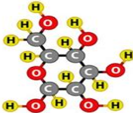
Glucose ( C_6H_{12}O_6 )
