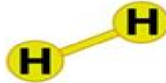
Hydrogen ( H_2 )
