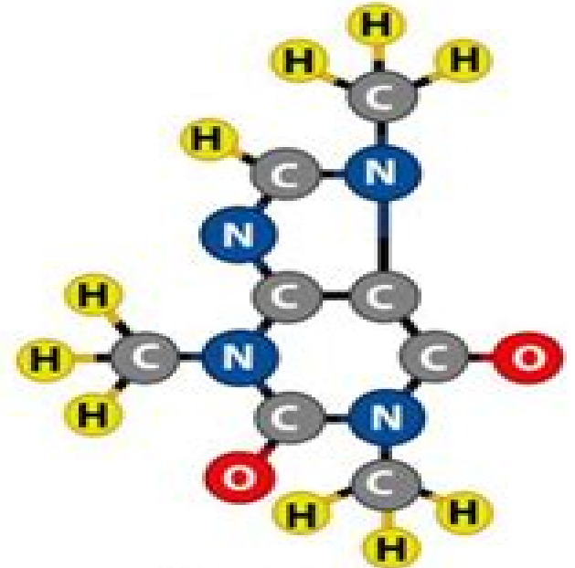
Caffeine ( C_8H_{10}N_4O_2 )
