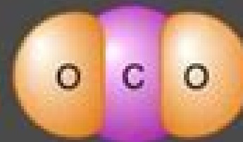
CO_2 carbon dioxide
